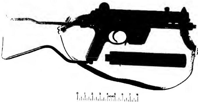
Figure 57. 9 mm MPK Walther Submachine Gun and West German Silencer
